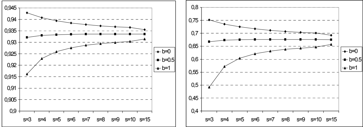
Example 3: n = 100 , n_c = 60 , K = 15 , q = 0.8 Example 4: n = 100 , n_c = 60 , K = 40 , q = 0.8
